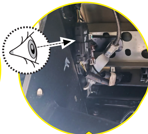
TAILGATE CONNECTOR
